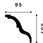
AT NOMASTYL® 100 x 95 x 2000 mm ART.NR. 3003162 EAN 5412938509497
