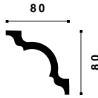
A1 NOMASTYL® 80 x 80 x 2000 mm ART.NR. 3003159 EAN 5412938509442
