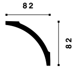
B8 NOMASTYL® 82 x 82 x 2000 mm ART.NR. 3007246 EAN 5412938954280
