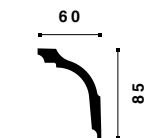
GL NOMASTYL® 85 x 60 x 2000 mm ART.NR. 3028323 EAN 5412938979429
